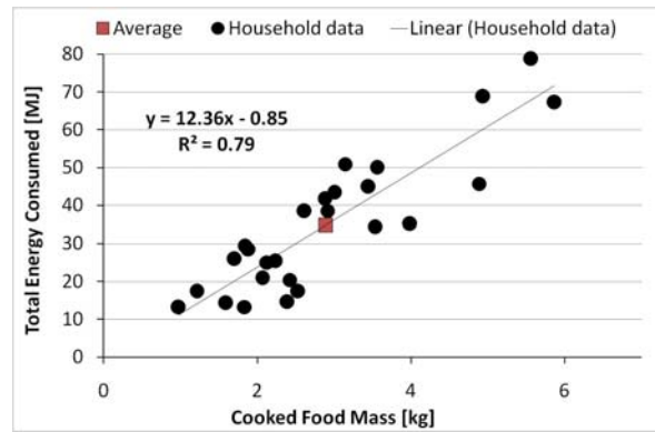
Figure 1: Specific Fuel Consumption (no char case) – the relationship between Total Energy Consumed and Cooked Food Mass
